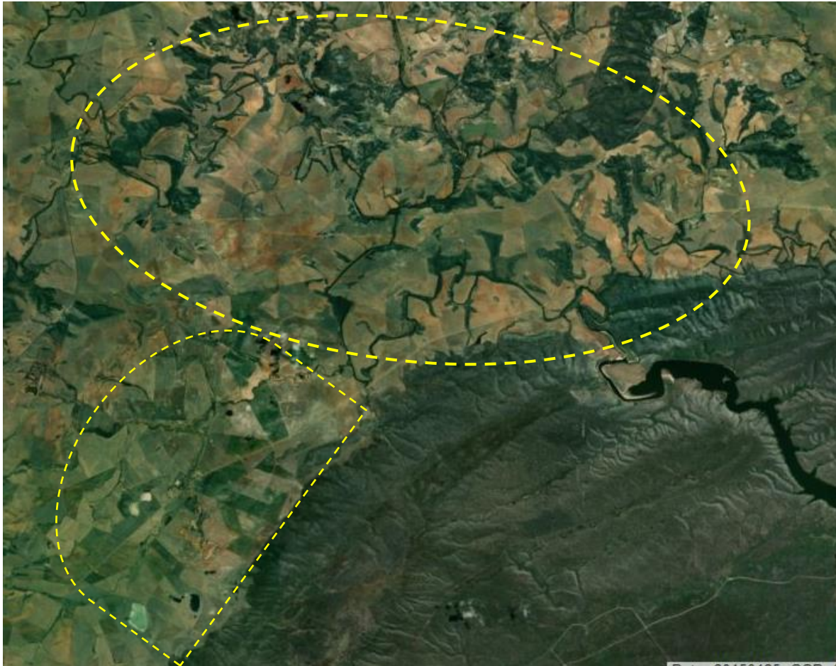
Figure 22. Satellite image showing the Enon Formation deposits in the Soutpansvlakte Basin (dashed half-moon, as in Figure 16) and in the northeast extension (dashed ellipsoid).
