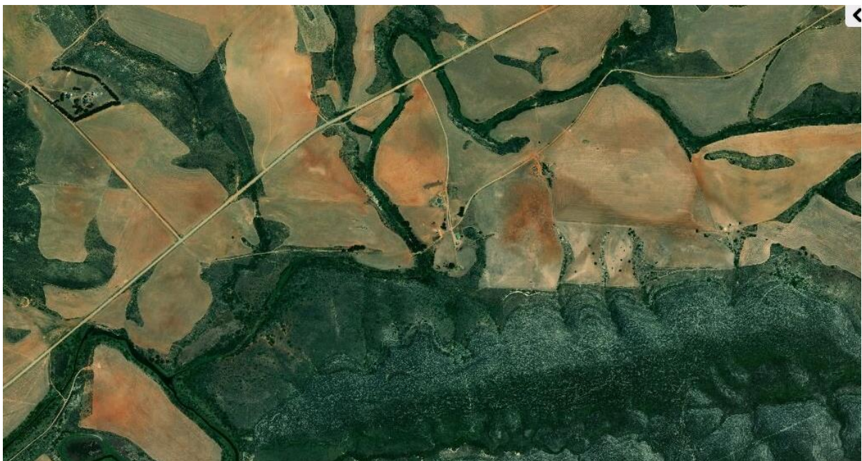
Figure 19. Enon Formation deposits east of the Soutpansvlakte Basin (the Kathoek Farm buildings are at the centre of the image).
