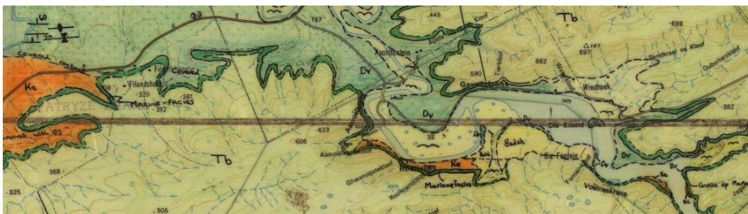
Figure 1. Geology map showing Enon Formation deposits in the Soutpansvlakte Basin (top) And in the Salt River Gorge (bottom).
