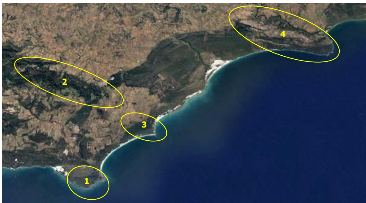
Figure 1. Satellite image showing the locations of the four TMG Formations outcrops in the Study Area: 1 – Agulhas; 2- Bredasdorp; 3 – Arniston; 4 – Potberg.
