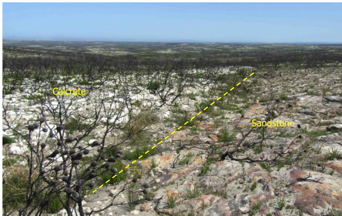
Figure 30. Top and bottom: the contacts between calcrete and sandstone (dashed line). The ground is exposed after a fire, which burnt the entire vegetation in the area in December 2018.
