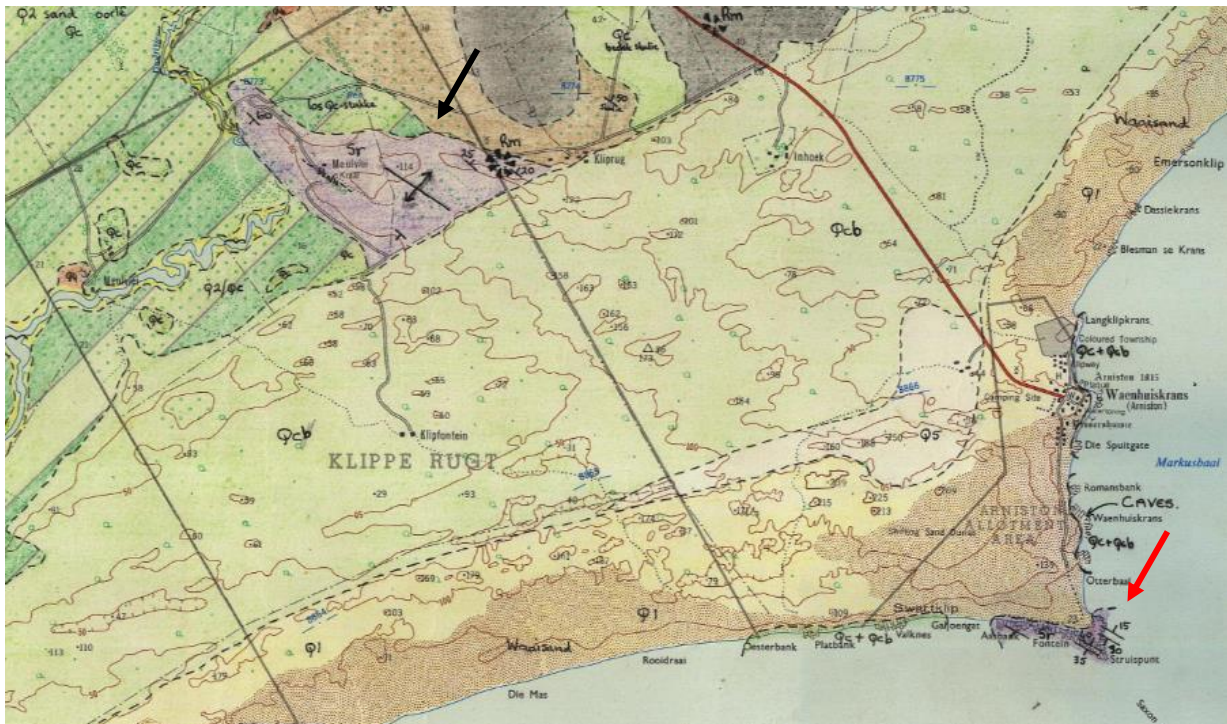
Figure 8. Geology map (Geological Survey field sheet, J Malan, 1984) showing the Arniston outcrops. Black arrow – Meulvlei Ridge; red arrow – Struis Point. The presence of the Reitvlei Formation rocks between the outcrops indicates possible buried ridge. (Note that ‘Klippe Rugt’ is the name of the parent farm, which may refer to the Meulvlei Ridge).
