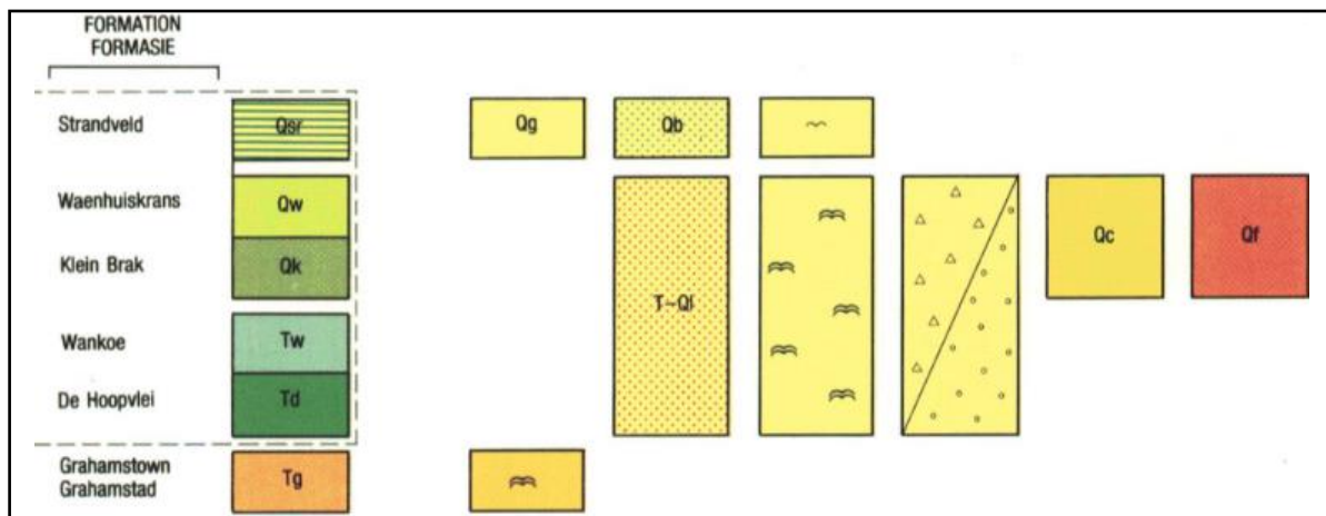
Figure 6. Legend of the Riversdale 1:250,000 geology map of 1990. Top - top section of the legend; bottom – legend extension to the right. The symbol of the Grahamstown Formation is Tg:
