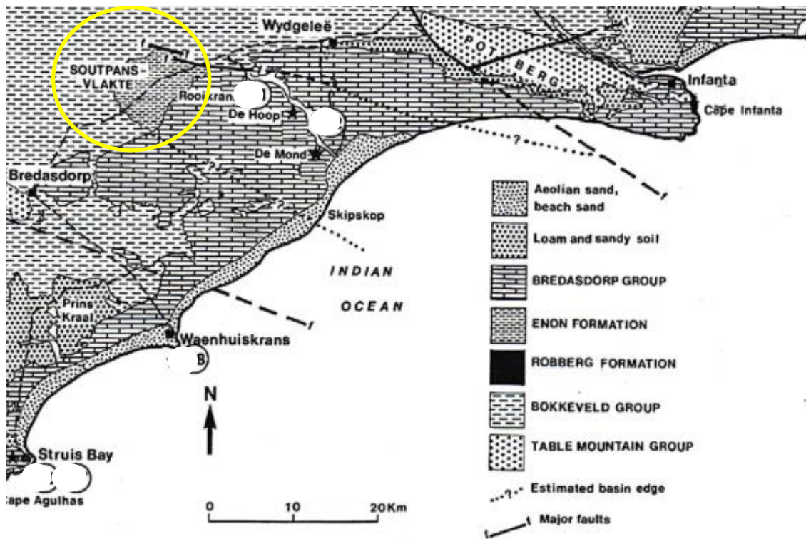
Figure 1. Generalised geology map of the study area. The circle indicates the area in question. The limestone of the Bredasdorp Formations was deposited over the Enon Formation. (Modified; from Field Trip Guide, 2016, by J Malan and J Viljoen).
