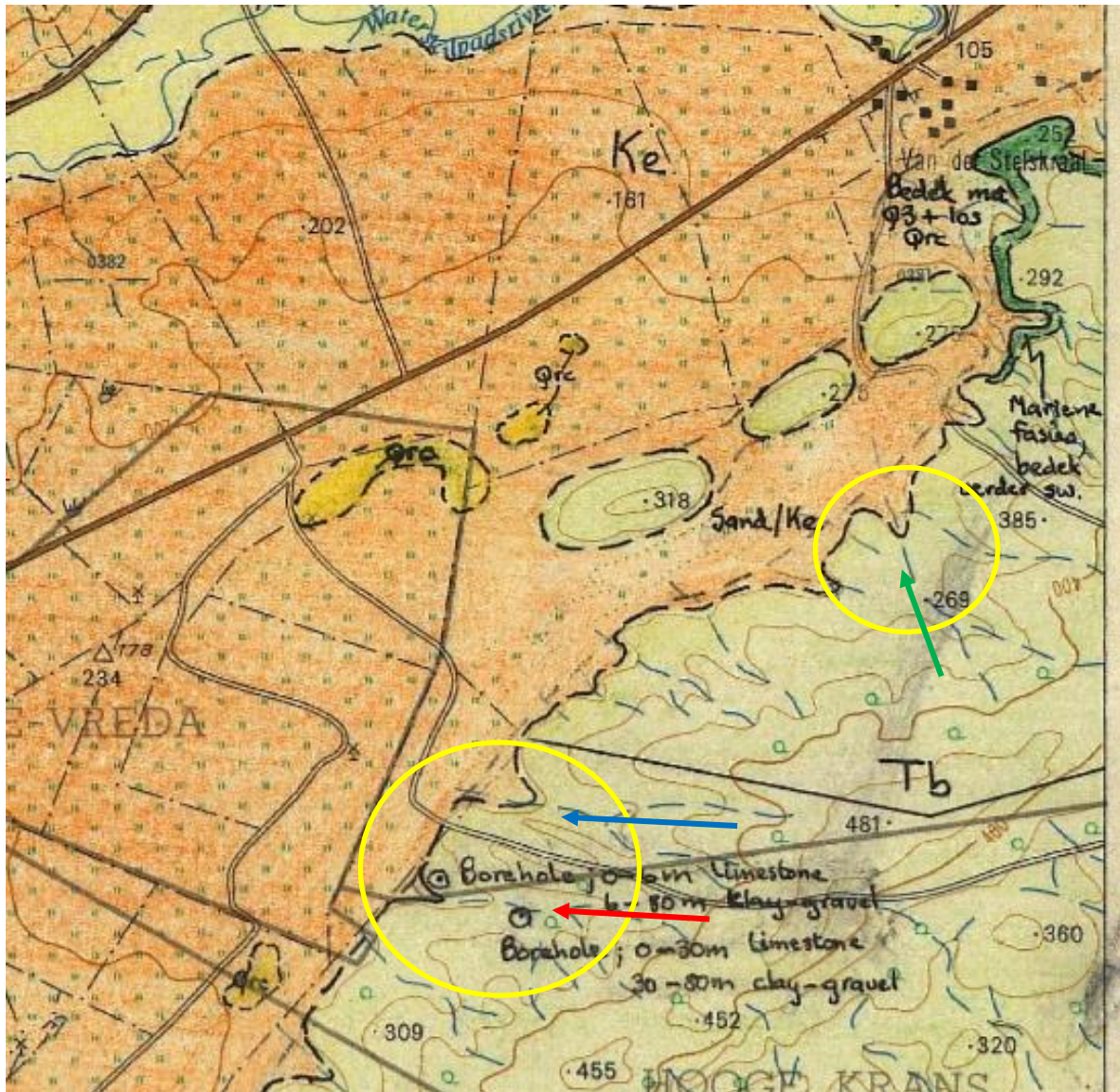
Figure 8. Geology of the area (from geology map 3420AC, field-sheet of 1984, at 1:50,000; elevations in feet). The light-green colour represents the limestone of the Hard Dunes (Bredasdorp Group); the orange colour represents the Enon Formation deposits. The circles indicate the borehole areas. Arrows point to the ravines, where the boreholes are situated. Note that the map is from 1984 and some features (roads etc) have changed since.
