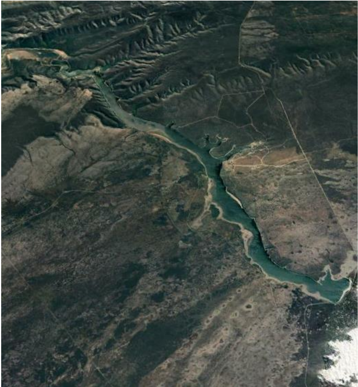
Figure 1. Satellite image of the De Hoop Vlei Gorge area.
